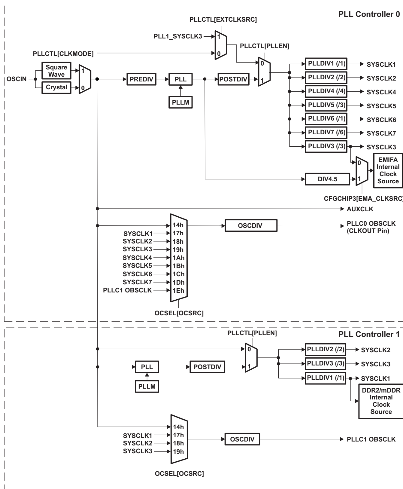
Figure 5-9. PLL Topology
