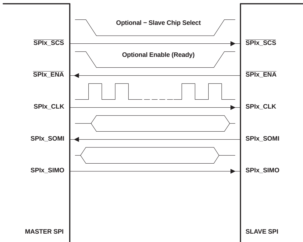
Figure 5-37. Illustration of SPI Master-to-SPI Slave Connection
